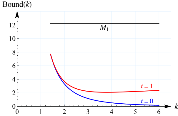
Figure 1: Bounds obtained by Theorem 1 when \sqrt{2} \leq k \leq 6 : Case (a) for t = 0 and t = 1
