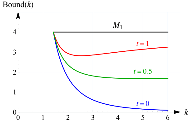
Figure 2: Bounds obtained by Theorem 1 when \sqrt{2} \leq k \leq 6 : Case (b) for t = 0, 1/2, 1
