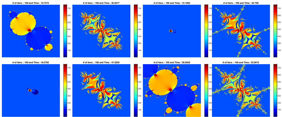
Figure 13: Example 4.7 for \alpha_n = \alpha_n^1 = \alpha_n^2 = \alpha_n^3 = 0.1 for all n \in \mathbb{N}_0 , \theta = 0.9 , accuracy \text{eps} = 1 , the area being [-20, 20]^2 , the iteration count fixed at 100 and \omega = 0.009 : (from left to right): Algorithms CJP, JPI (ver. 2), CJM, JMI (ver. 2) (first line); Algorithms CJI, JII (ver. 2), CJNS, JNSI (ver. 2) (second line)
