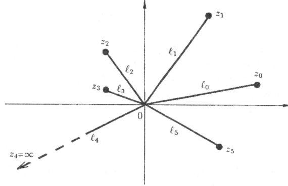
Figure 2.1: The rays in the complex plane ( M = 6 )
